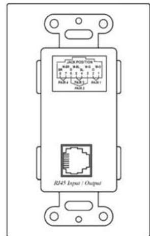
Rear View
