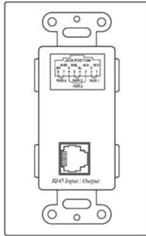
Rear View
