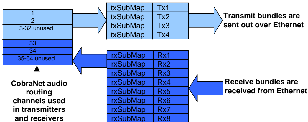
Figure 3. Mapping of ASI2202 inputs and outputs to CobraNet channels.
